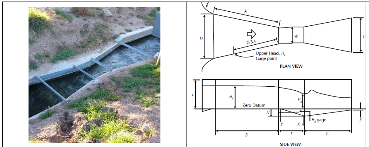
Figure 2-10: Standing-wave Parshall Flume – Field Installation and Schematics
